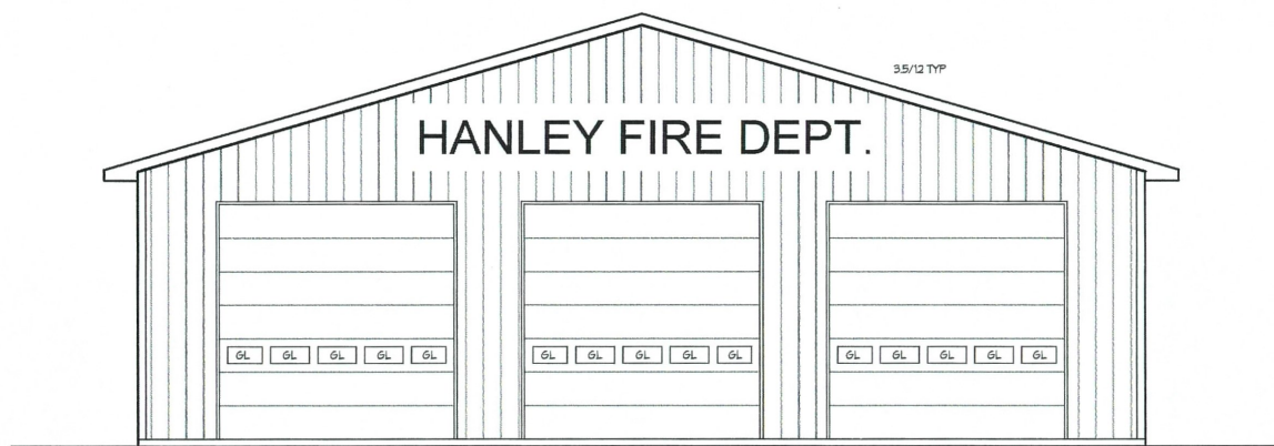
2 FRONT ELEVATION 1/8"=1'-0" - 1504C
